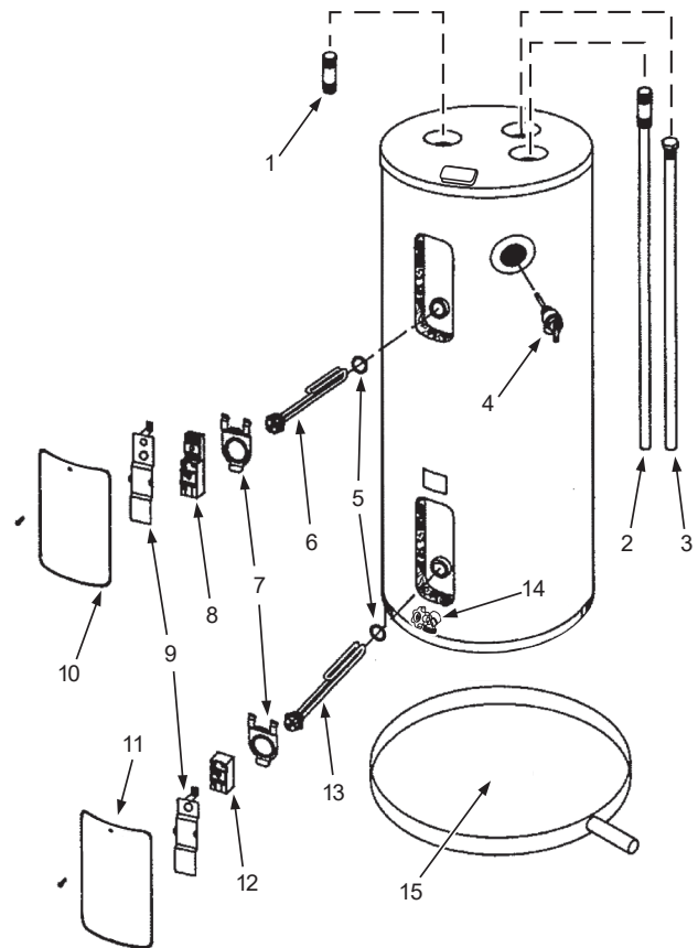
Figure 7. Repair Parts
